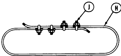
DETAIL 4
