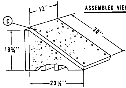
ASSEMBLED VIEW
