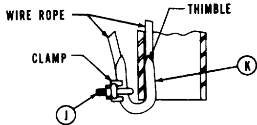
DETAIL 5
