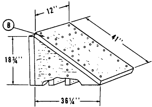
ASSEMBLED VIEW
